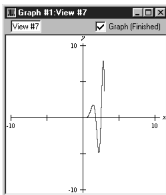
Figure I.16: Graph of Relation #1 with two constraints
