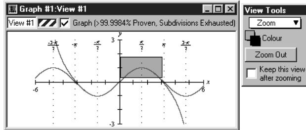
Figure II.10: Zoom box on the curves, and where x=\pi/2
