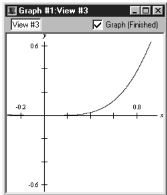
Figure I.13: Graph of the edited Relation #1
