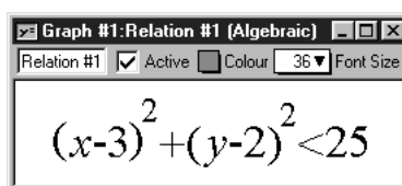
Figure I.17: Relation #1 for the simultaneous system
