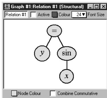
Figure 3.1: A structural relation window displaying y=\sin x
