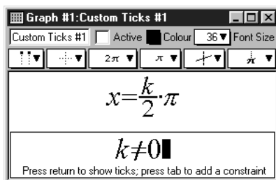
Figure II.8: Custom ticks in multiples of \pi/2
